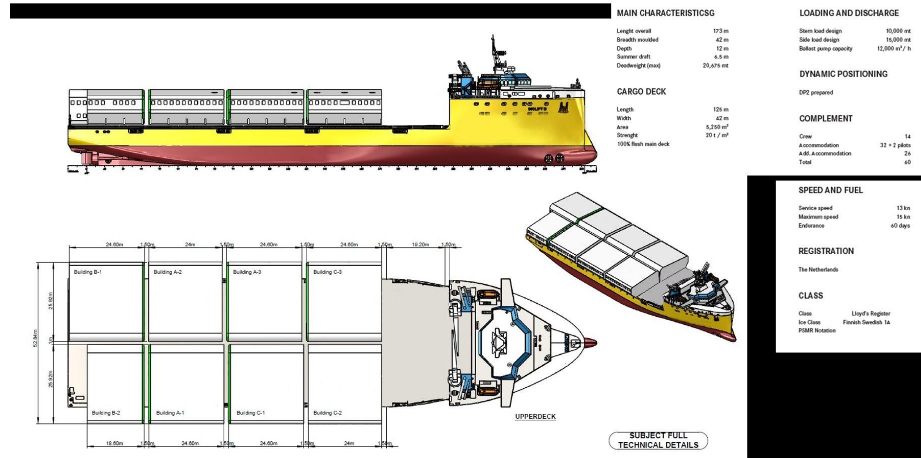
Figure 47: Preliminary loading arrangement and characteristics of the proposed MC Class vessel for the delivery of the building modules 18 .
