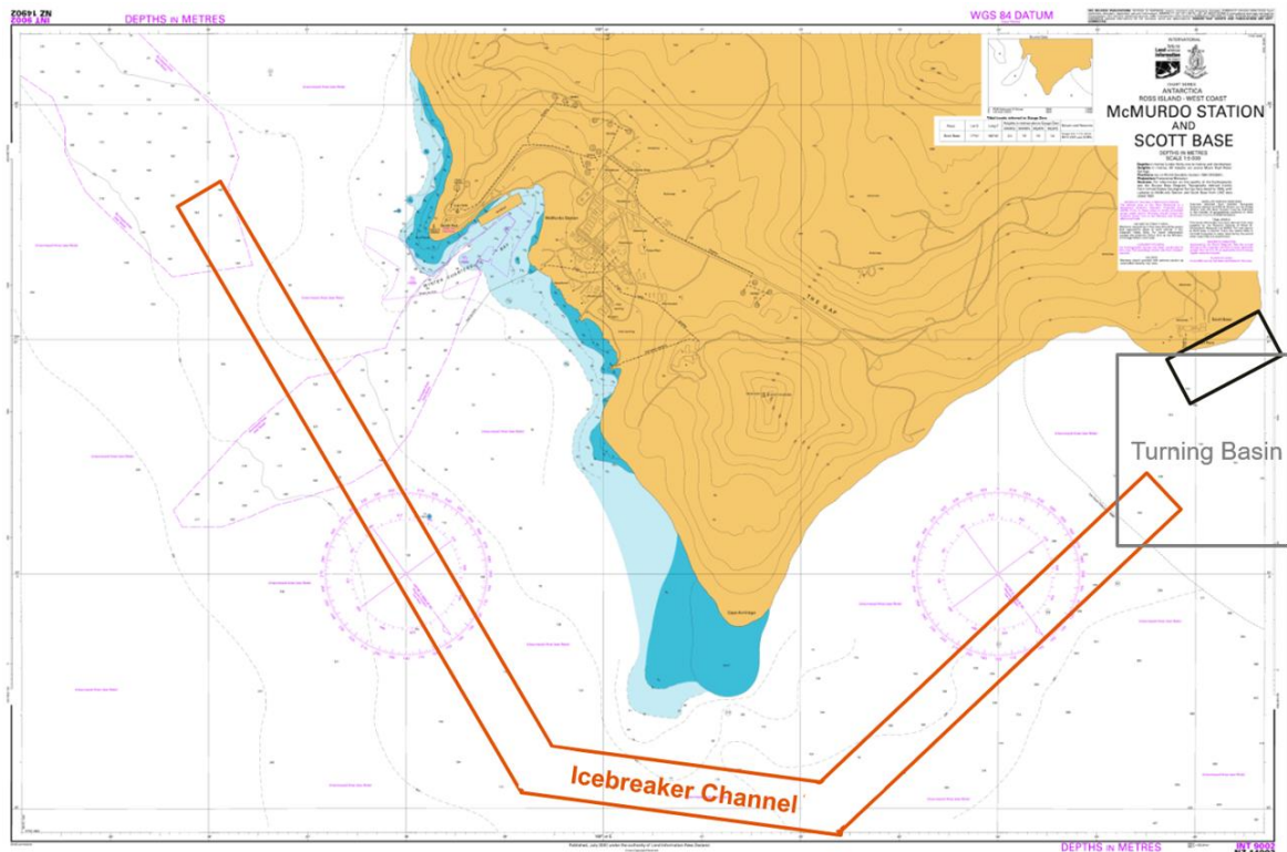
Figure 50: Indicative location of the additional icebreaker channel required to reach Pram Point.
