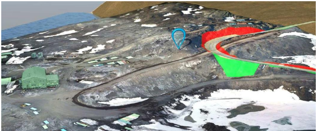
Figure 31: Proposed road realignment at the Scott Base transition. Red indicated cut and green indicated fill for the earthworks.
