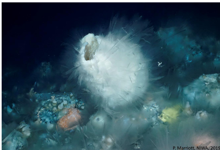
Figure 91: Anchor ice covering the seafloor at approximately 12 m depth at SB3. Animals of many types and sizes were covered by anchor ice at this depth. The large sponge (~50 cm tall) is Rossella racovitzae (Image: Peter Marriott, NIWA).
