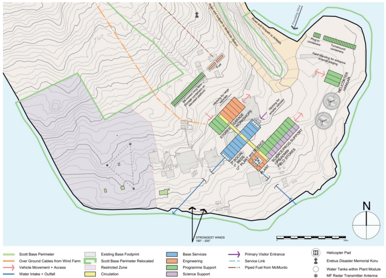
Figure 61: Concept Design C - plan view.
