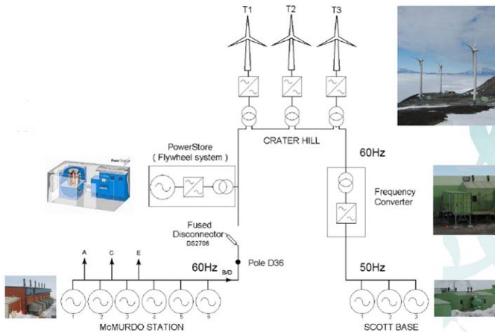
Figure 51: Current RIWE system design.
