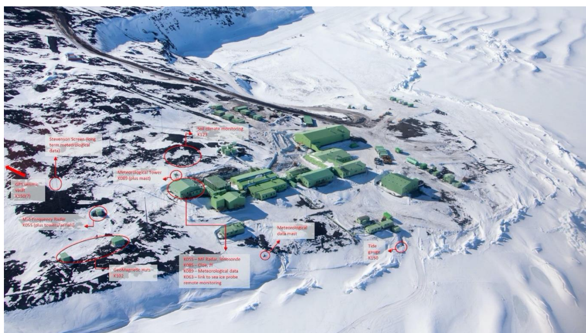
Figure 101: Long-term science installations at Scott Base
