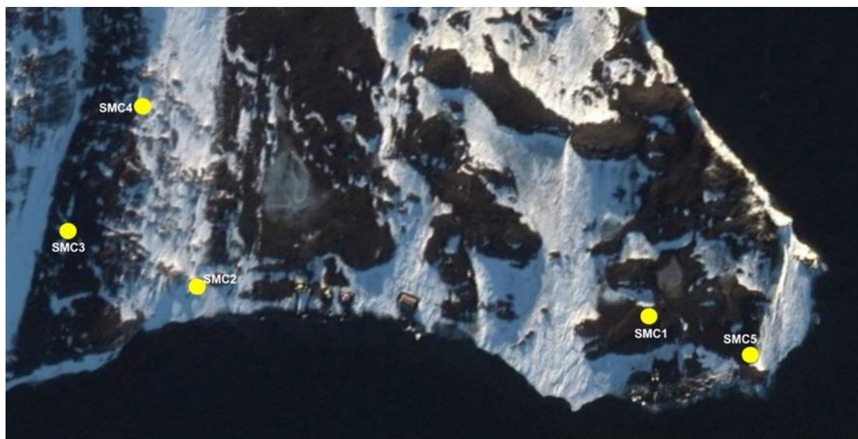
Figure 108: Location of the manually selected control sites at Cape Evans.
