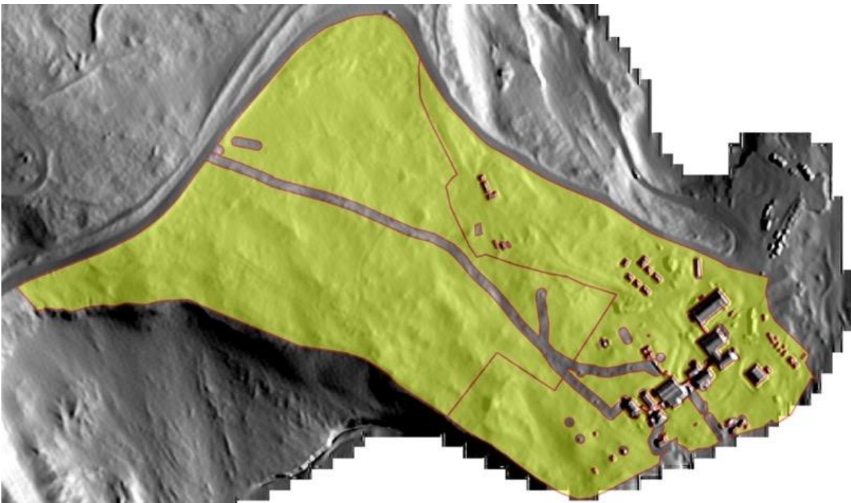
Figure 106: Identified region of interest for the baseline survey and terrestrial monitoring programme.
