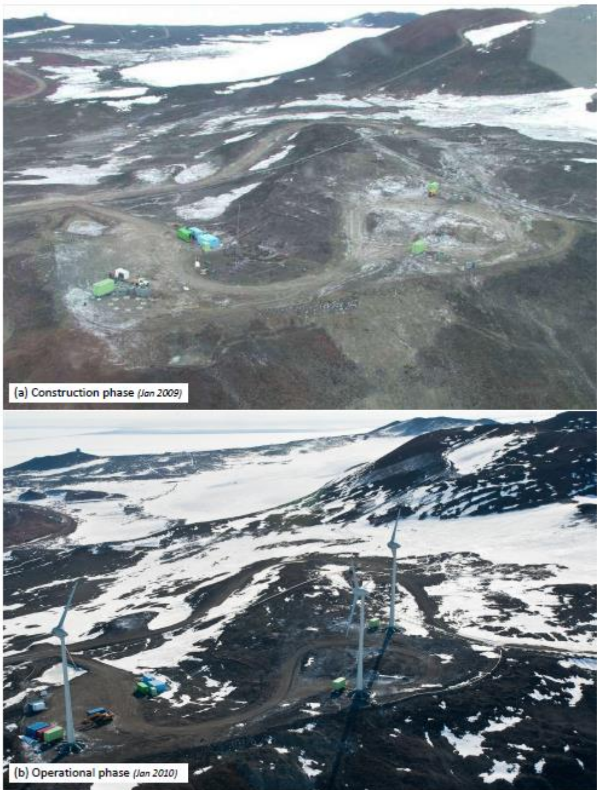
Figure 77: Aerial photo of the Crater Hill wind turbine site (New Zealand, 2008).
