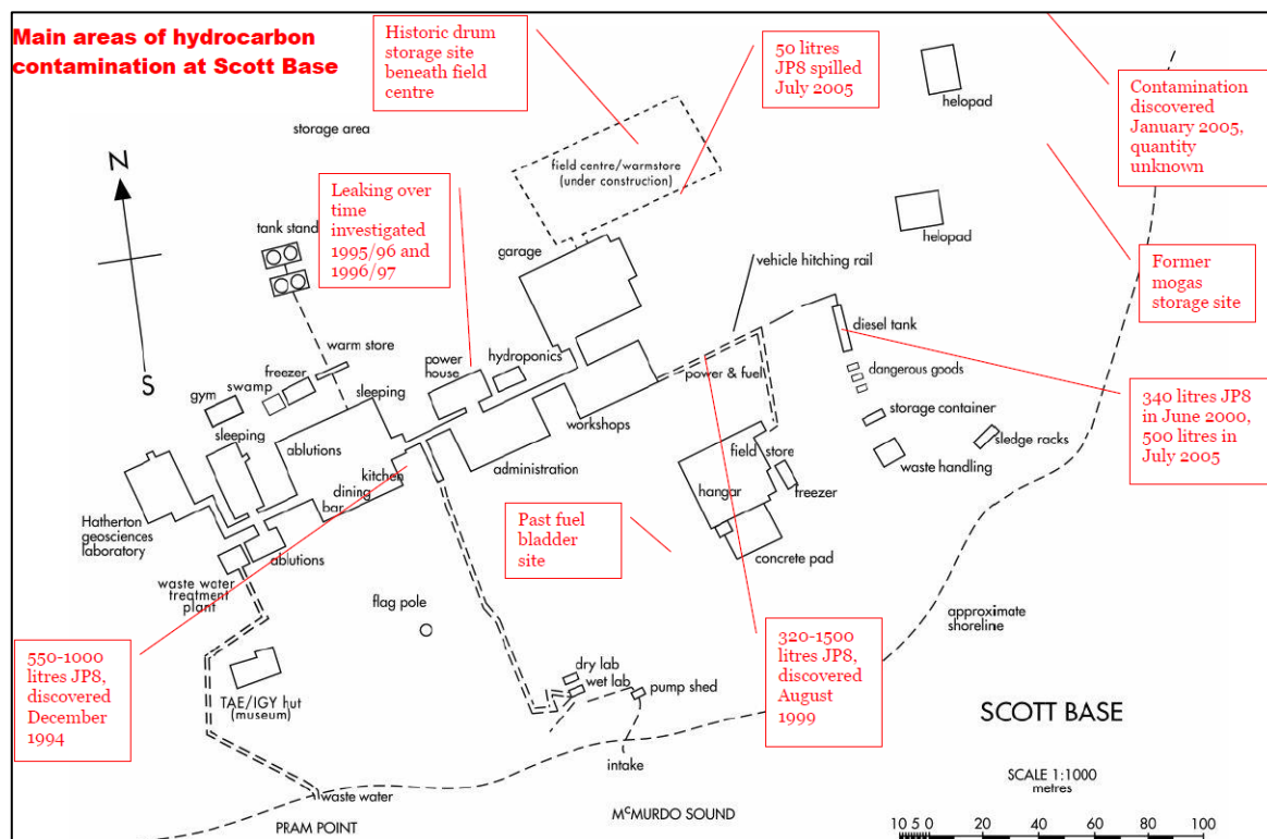
Figure 81: Known past contamination events within the Scott Base operational area.
