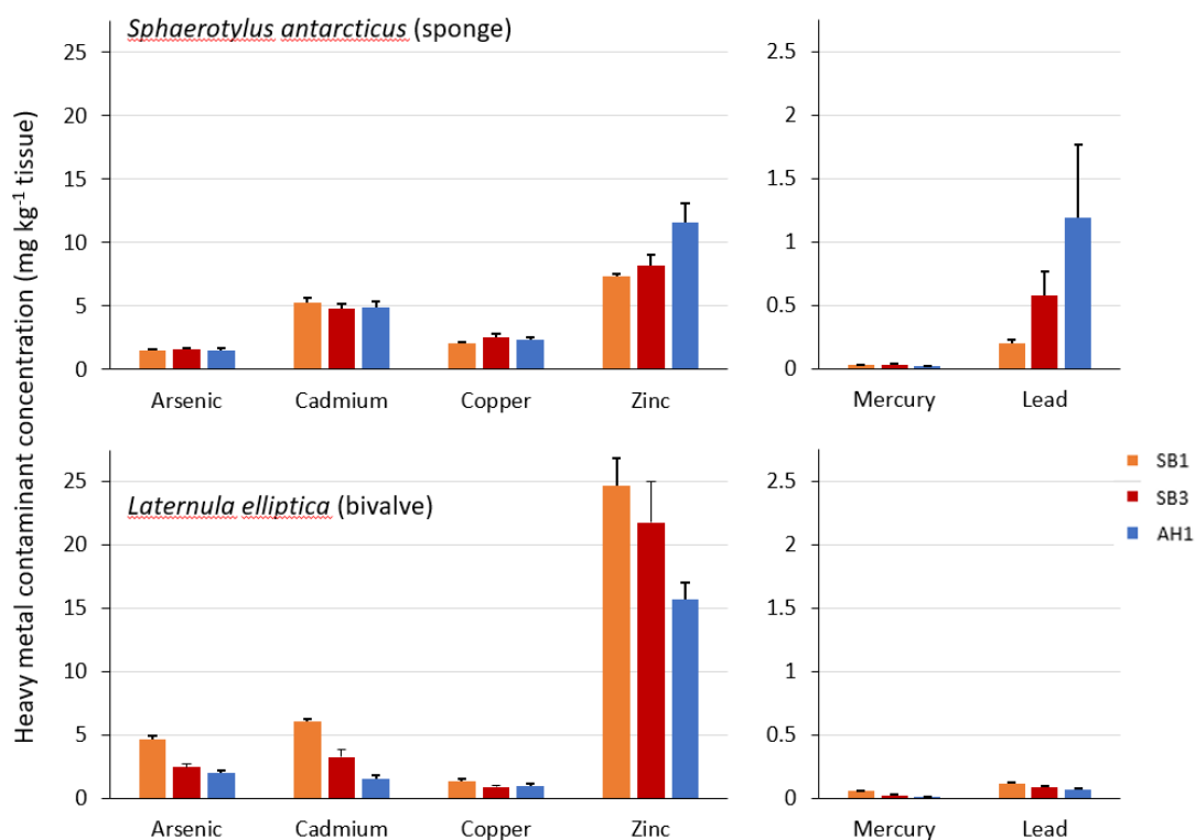
Figure 94. Heavy metal contaminant concentrations in sponge and bivalve tissue samples at SB1, SB3 and AH1 34 .
