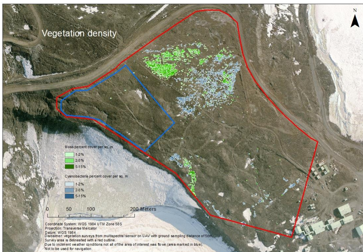
Figure 87: Vegetation cover at Scott Base from multispectral imagery (2018/19) 27 .
