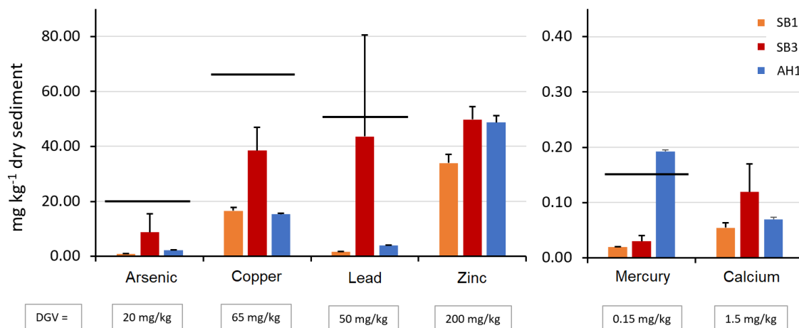
Figure 93. Sediment heavy metal contaminant concentrations at SB1, SB3 and AH1 33 .
