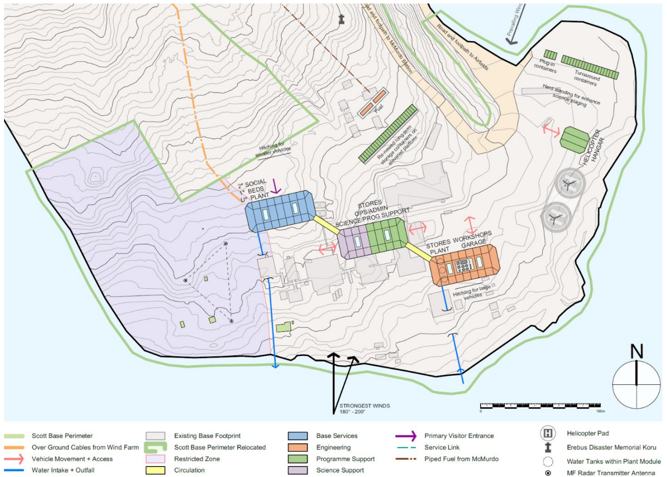
Figure 62: Concept Design D - plan view.
