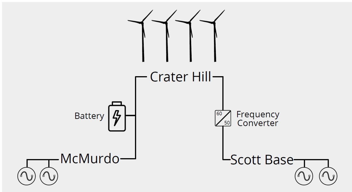
Figure 52: Power system concept design indicating from left to right, the McMurdo generators and distribution, the proposed BESS, proposed turbines, frequency converter, and Scott Base generators.
