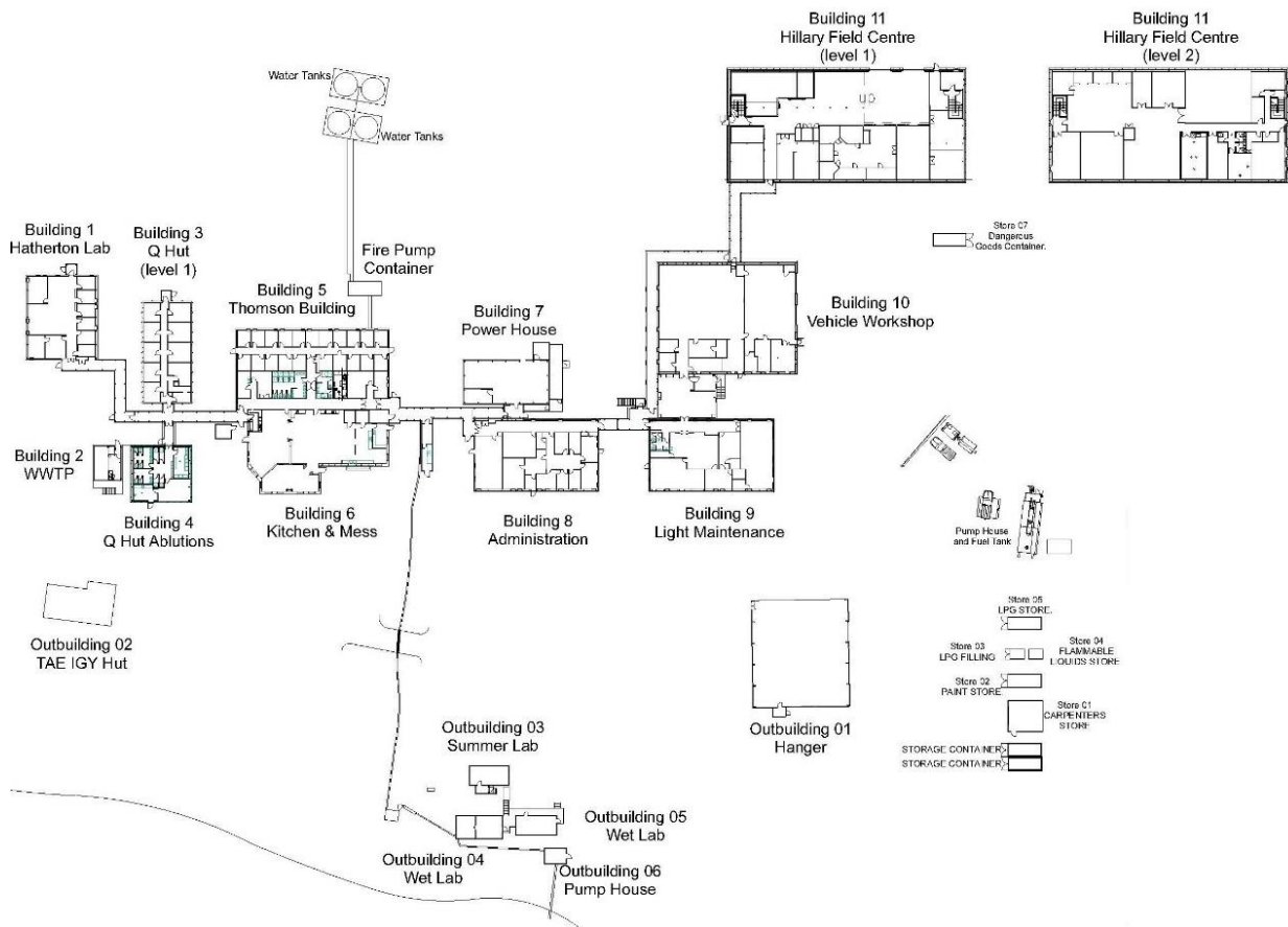
Figure 29: Current Scott Base building layouts for reference in the deconstruction methodology.
