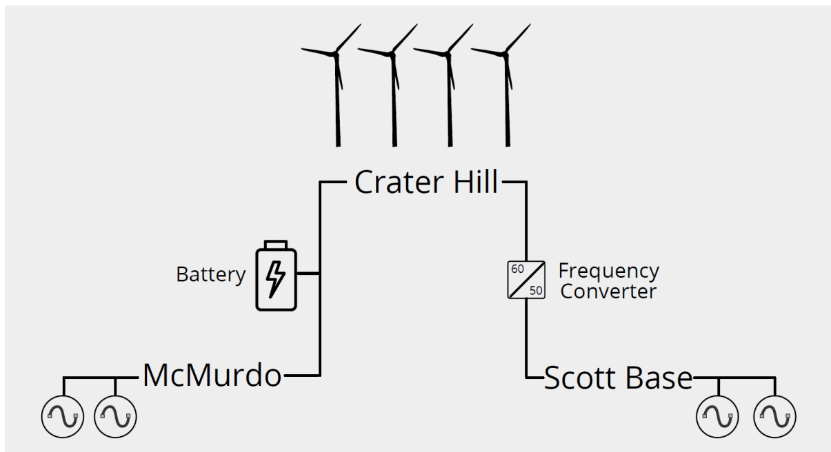
Figure VI: Power system concept design indicating from left to right, the McMurdo generators and distribution, the proposed BESS, proposed turbines, frequency converter, and Scott Base generators.
