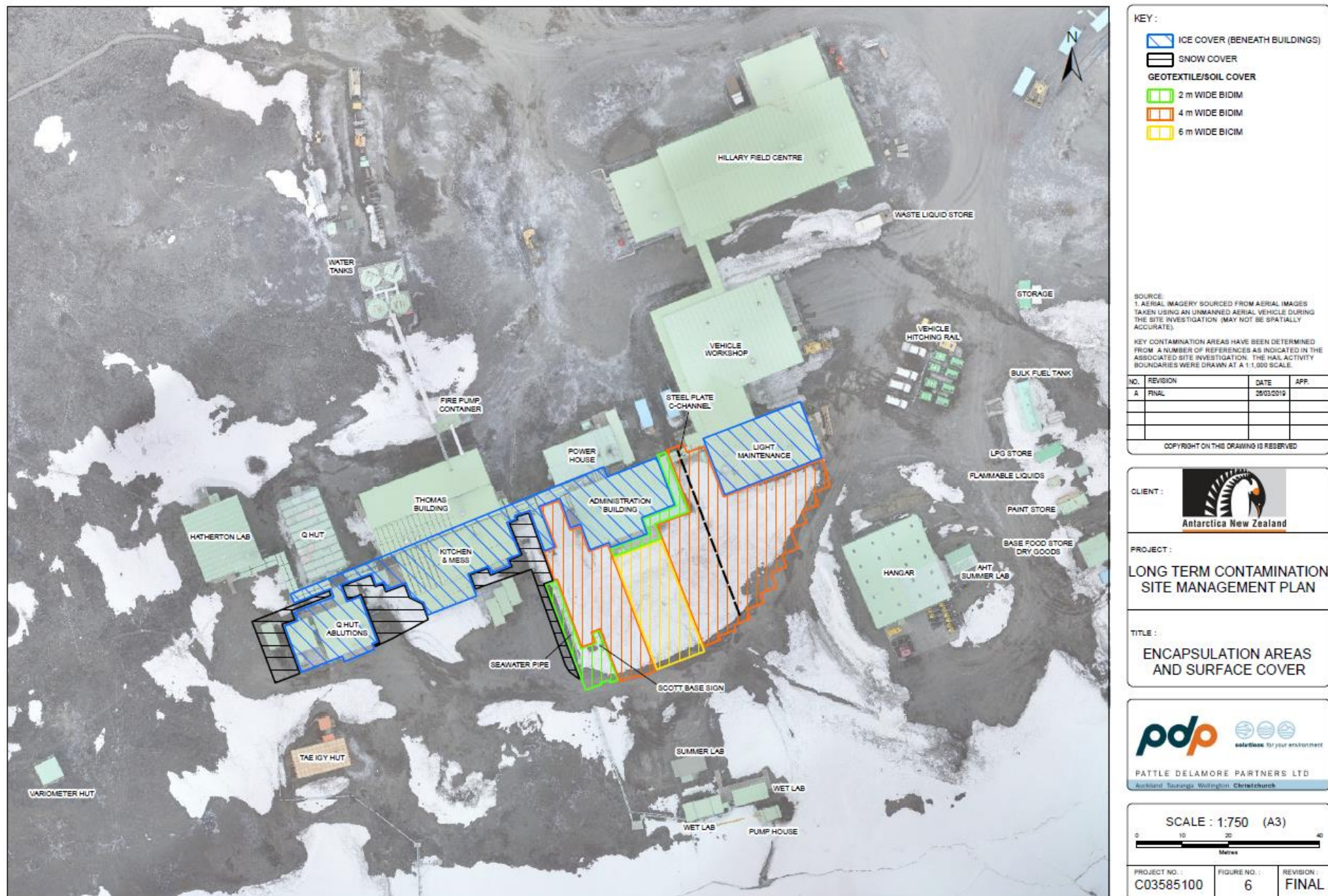
Figure 16 - Areas of encapsulation already at Scott Base.
