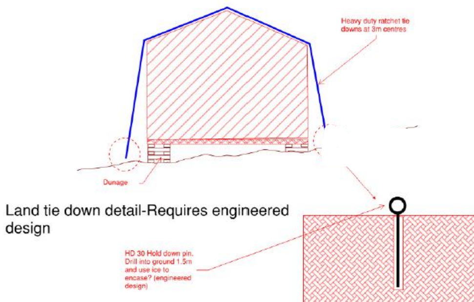
Figure 66: Land tie down detail for whole buildings stages for removal on ship.
