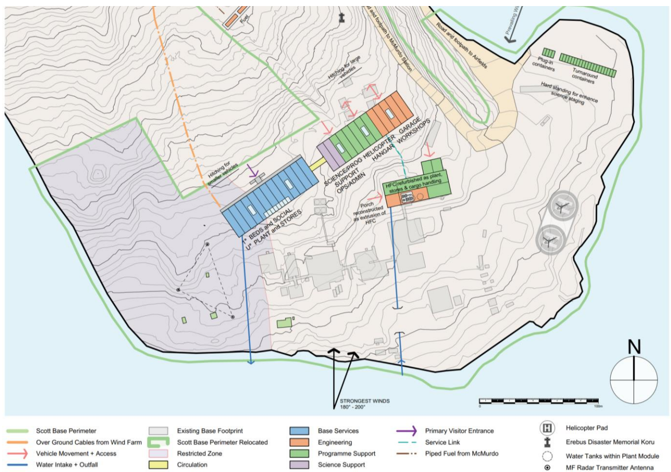
Figure 60: Concept Design B - plan view.
