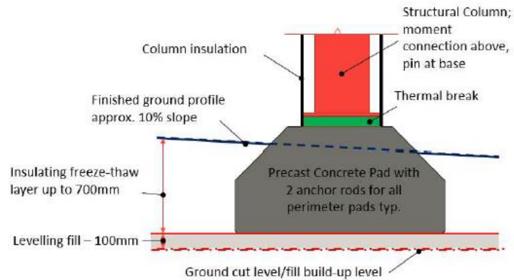
Figure 46: Concept pad foundations proposed for the Temporary Base buildings.
