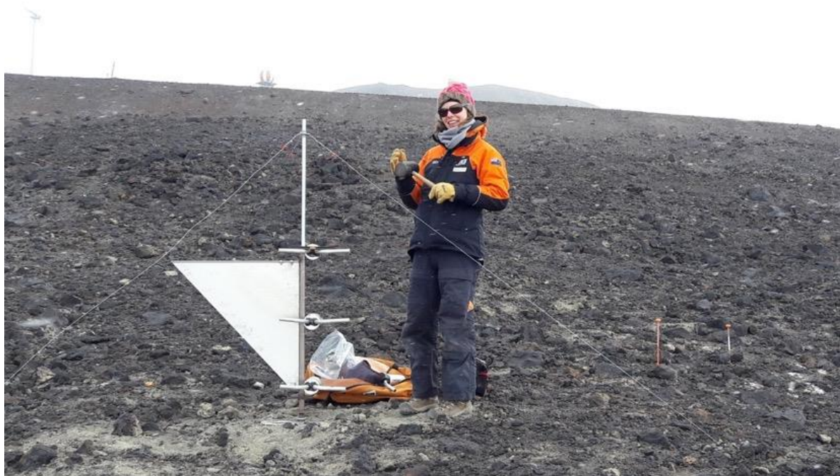
Figure 111: An MWAC dust sampler being installed at one of the monitoring sites behind the current Scott Base. Photo: O'Neill, University of Waikato.
