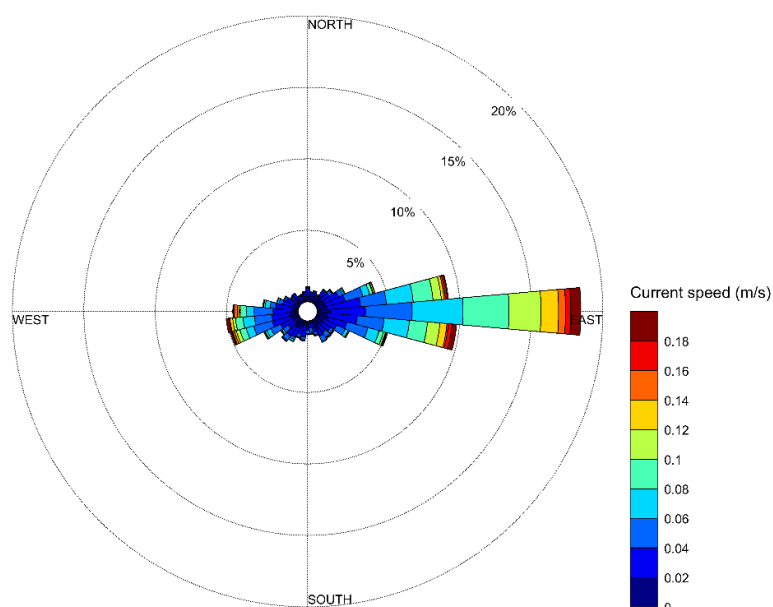
Figure 95. Current speed and direction at SB1 during November 2019. Distribution of depth-averaged current direction (degrees True) and velocity (m/s) between 28/10 and 18/11/19 35 .
