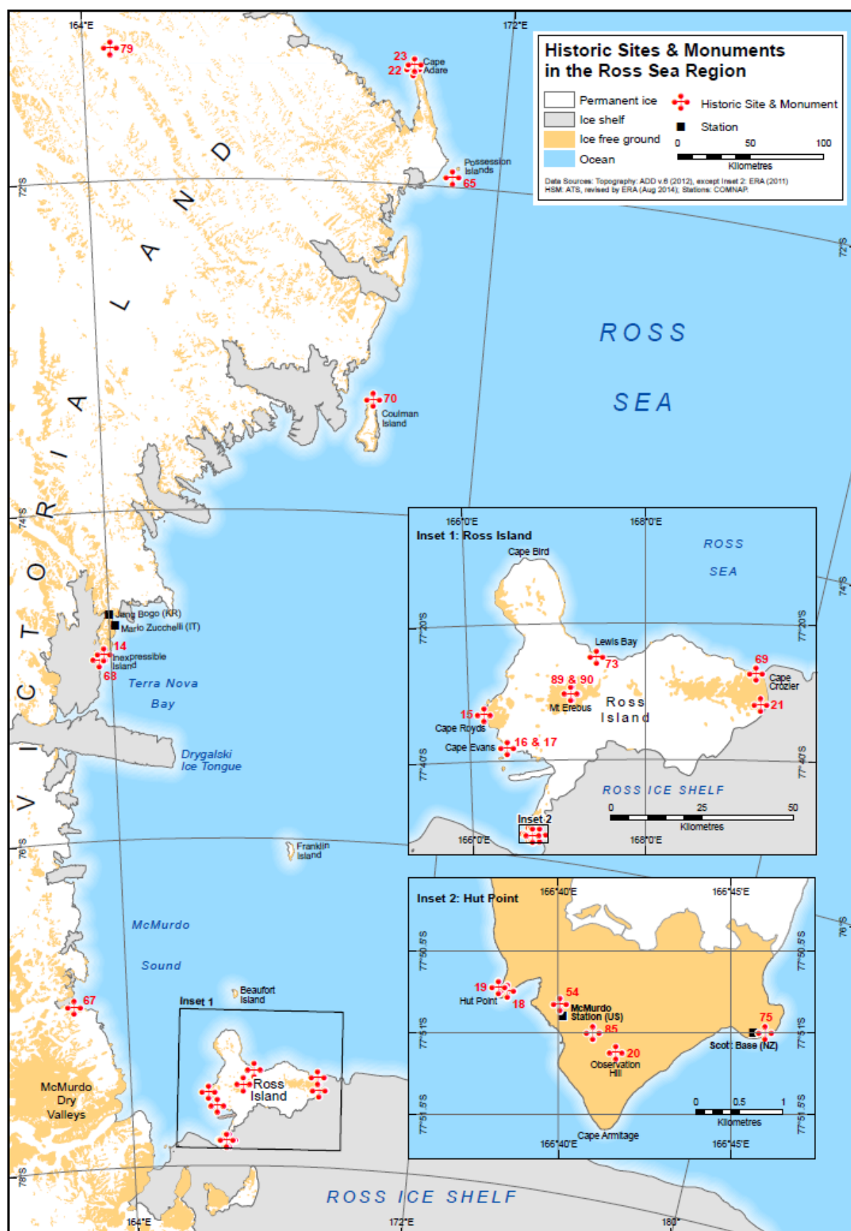
Figure 103: HSMs in the Ross Sea region.
