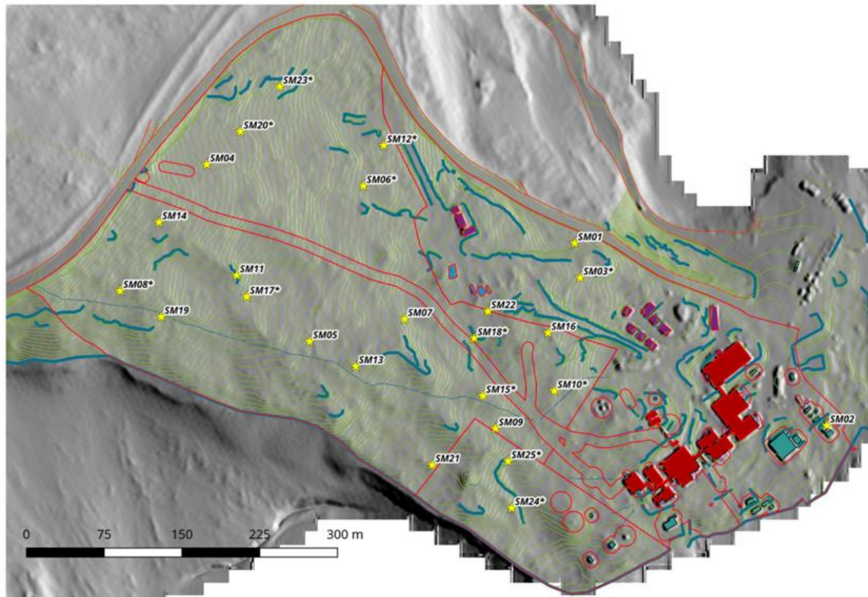
Figure 107: Map of the region of interest and the selected 25 terrestrial monitoring sites. * = MWAC dust sampler installed adjacent to the monitoring plot (see section 9.3.5). Source: (Roudier, 2019).
