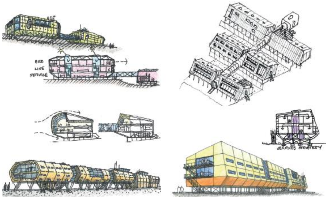
Figure 58: Concept sketches prepared during the early stage of design.
