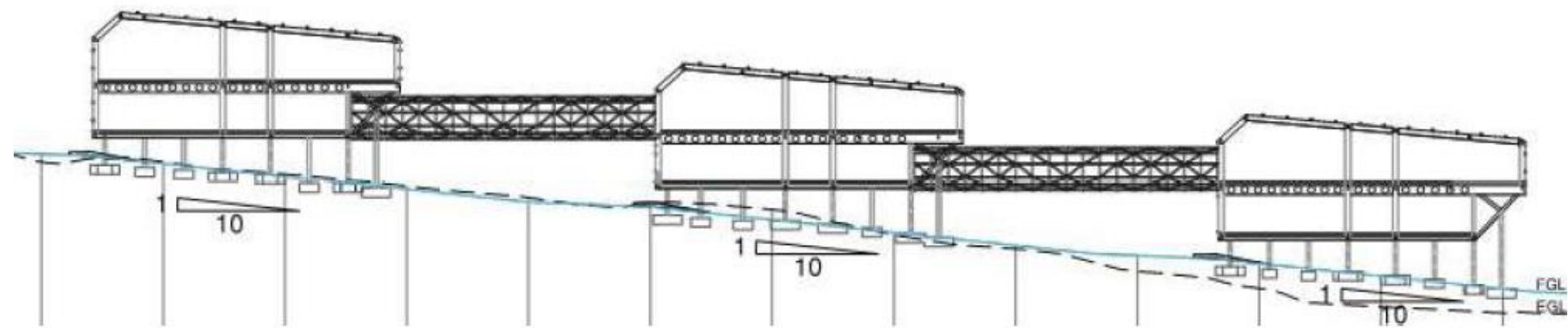
Figure 25: Proposed ground profile (blue line).
