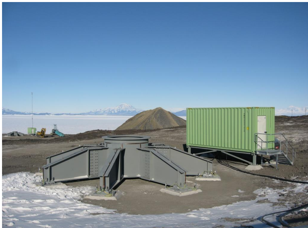
Figure 56: Steel spider framework bolted to the concrete foundation blocks.
