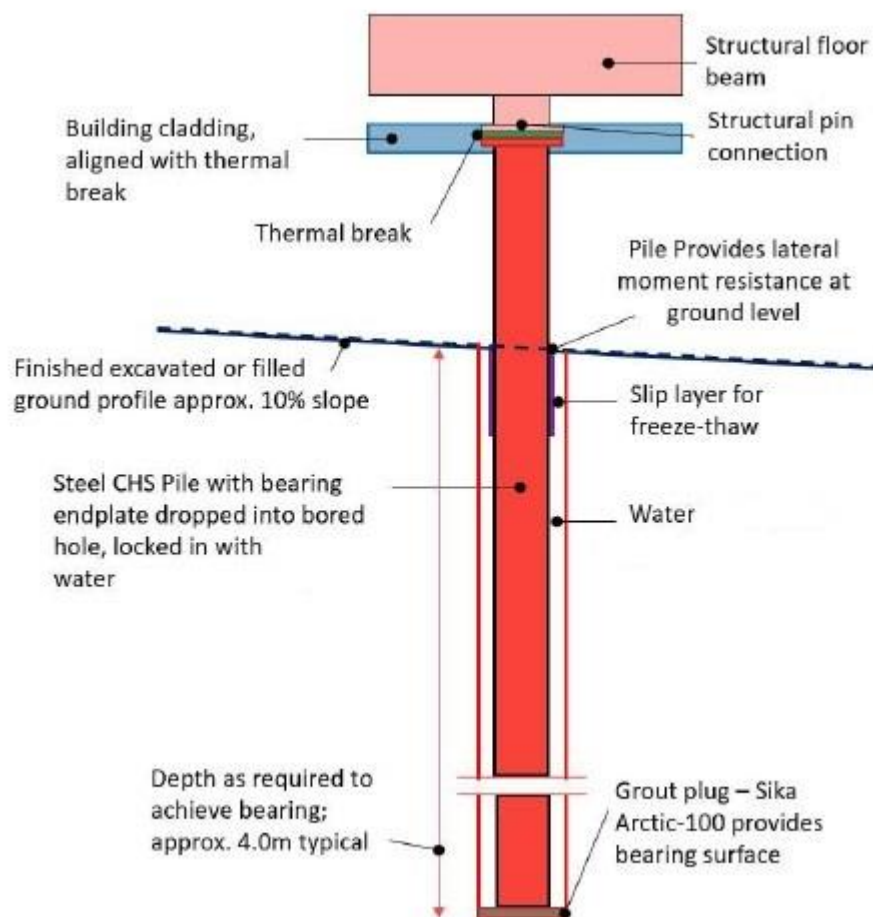
Figure 38: Sketch of the proposed end-bearing pile.
