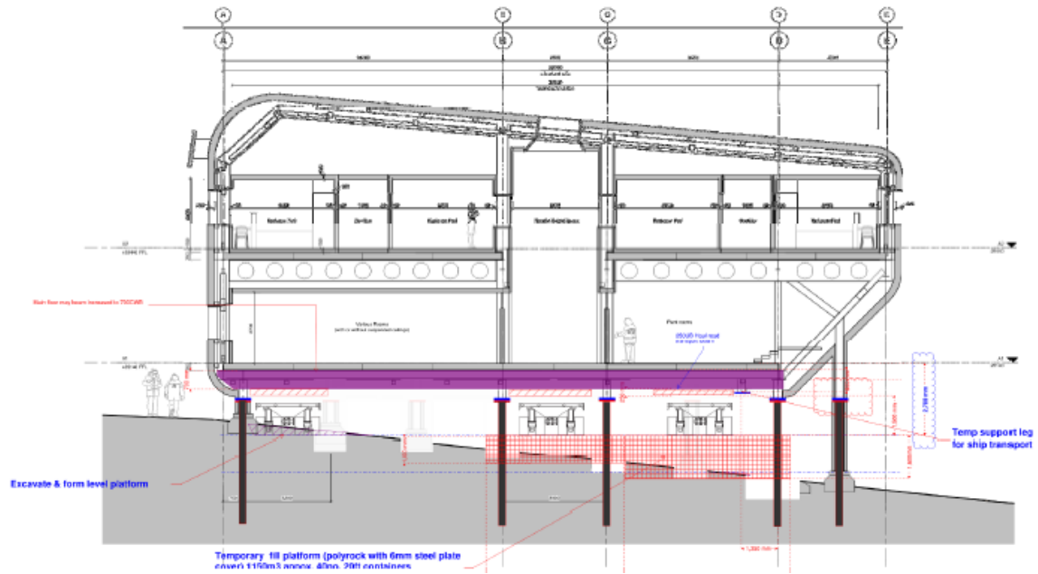
Figure 49: Side view of SPMTs delivering a building module to site. Red hash denotes the temporary platform due to gradient differences across the building platform.
