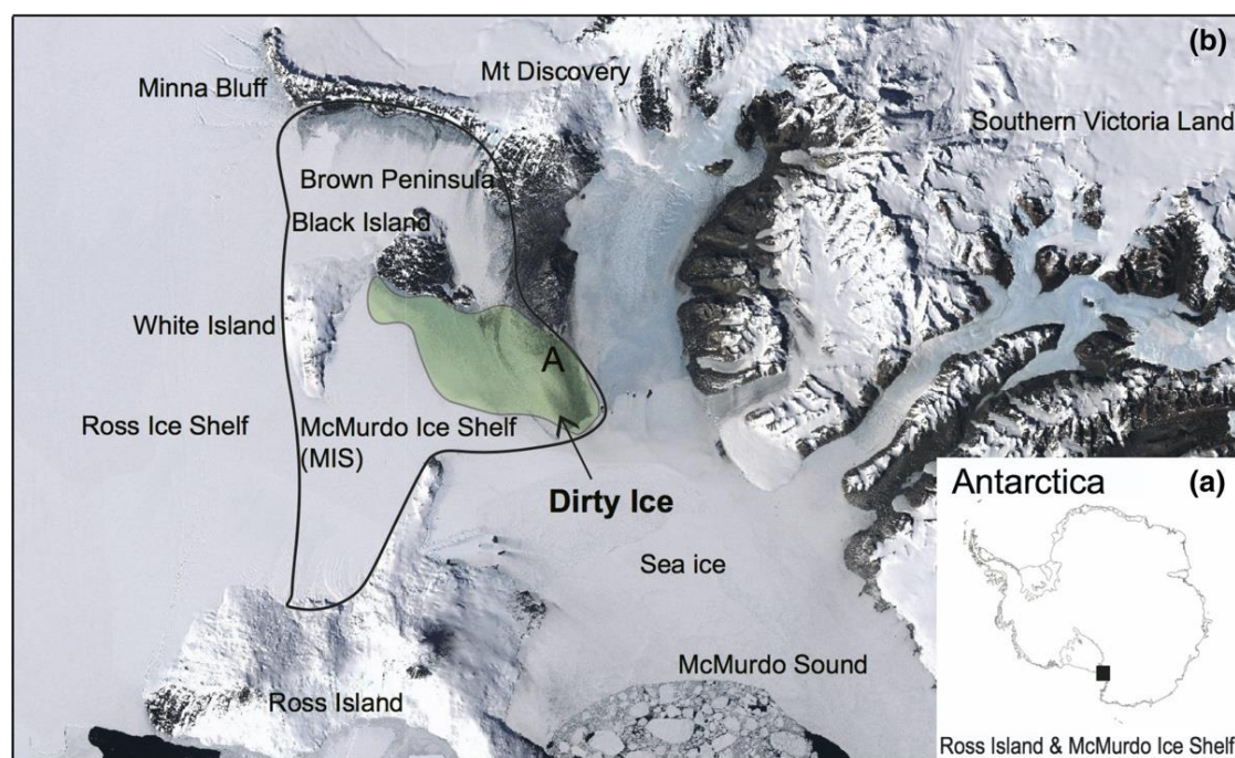
Figure 98: McMurdo Ice Shelf and Southern McMurdo Sound (Source: Hawes et al., 2018).
