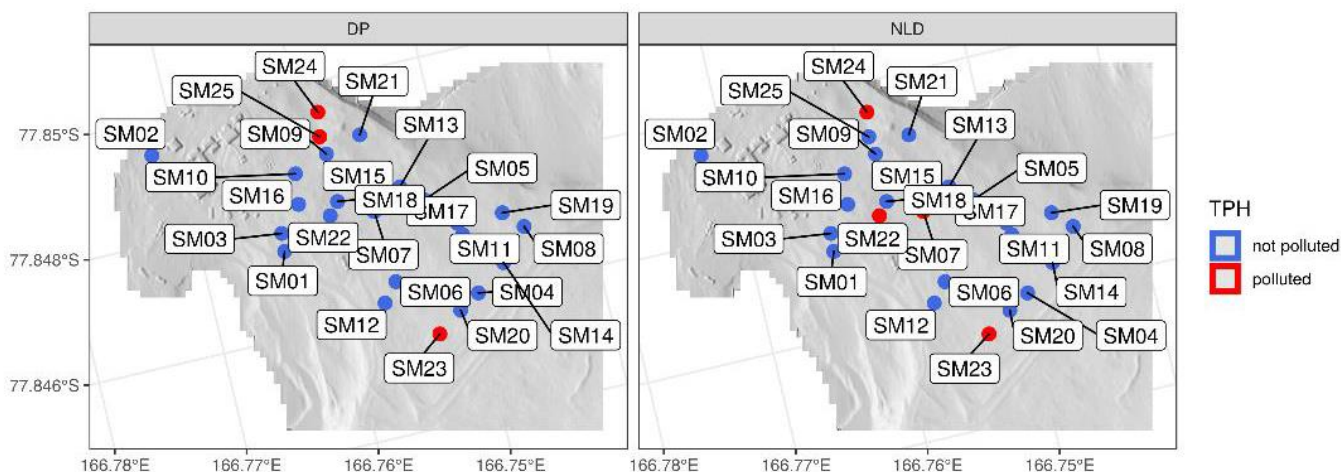
Figure 82: Estimated TPH contamination in surface soils (0-2cm) and soils at depth (2-10cm) at each of the soil monitoring sites above Scott Base.
