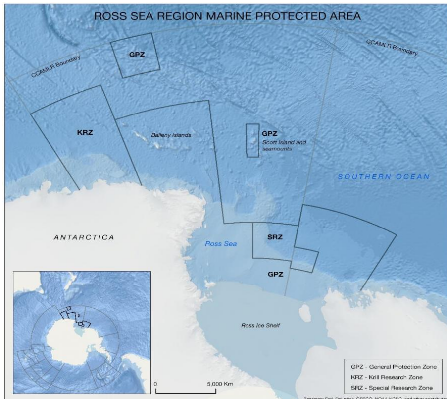
Figure 104: Ross Sea region Marine Protected Area.
