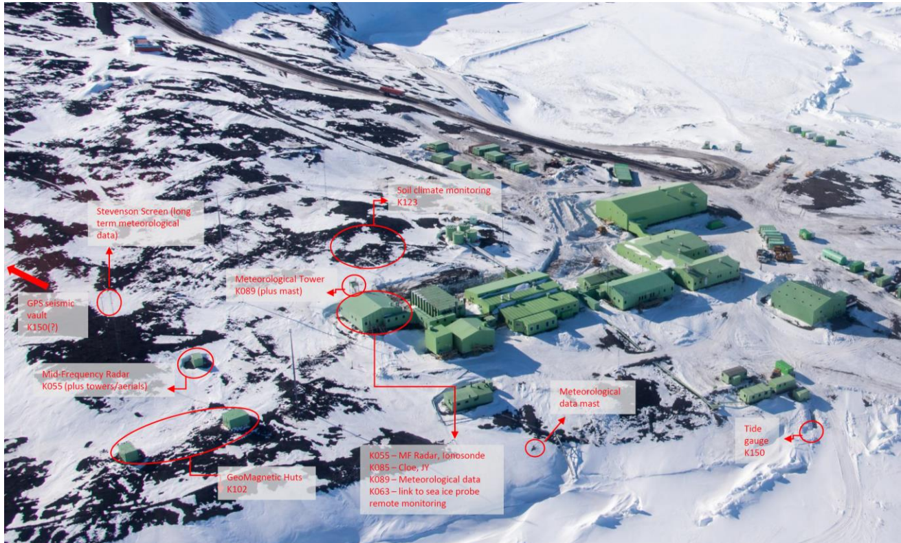
Figure 63: The location of long-term science experiments at Scott Base.
